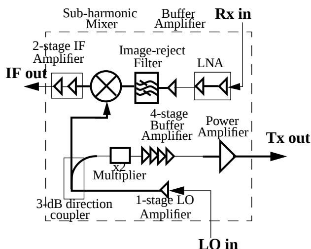
Figure 1 Block diagram of the transceiver MMIC using a subharmonic mixer.
